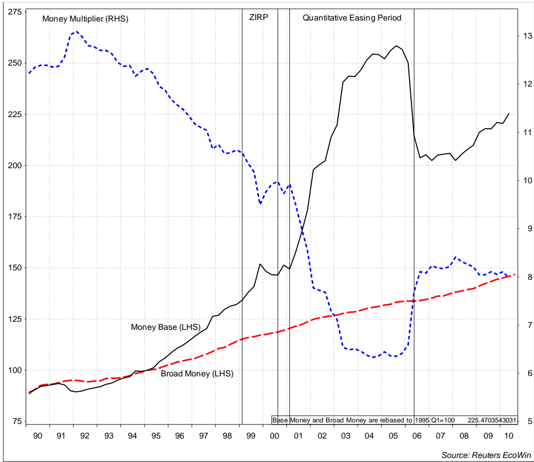
Figure 4: Money multiplier
