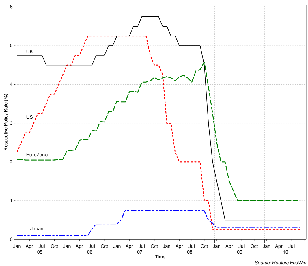
Figure 3: Policy rates
