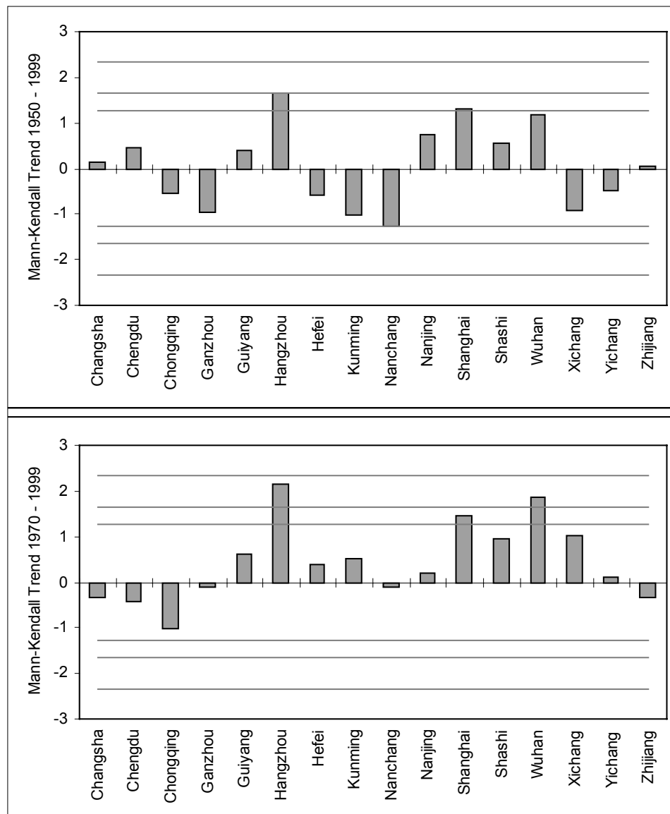
Figure 9: Mann-Kendall trend test for the inner-annual variability from 1950 to 1999 (upper graph) and from 1970 to 1999 (lower graph). The three lines above and below the abscissa represent the 90%, 95%, and 99% confidence levels of the trend tests.
