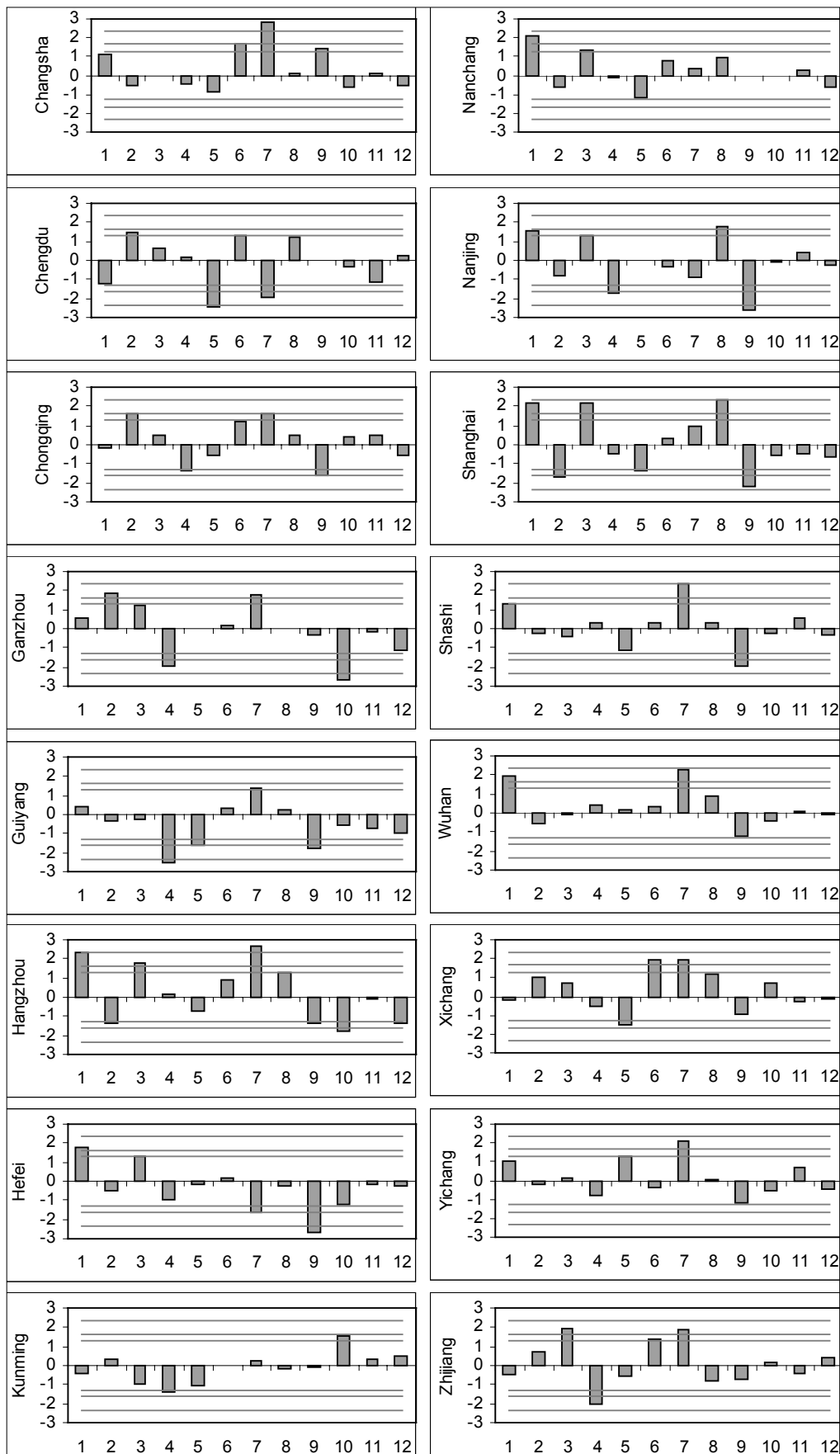
Figure 12: Mann-Kendall trend test for monthly precipitation 1970 – 1999
