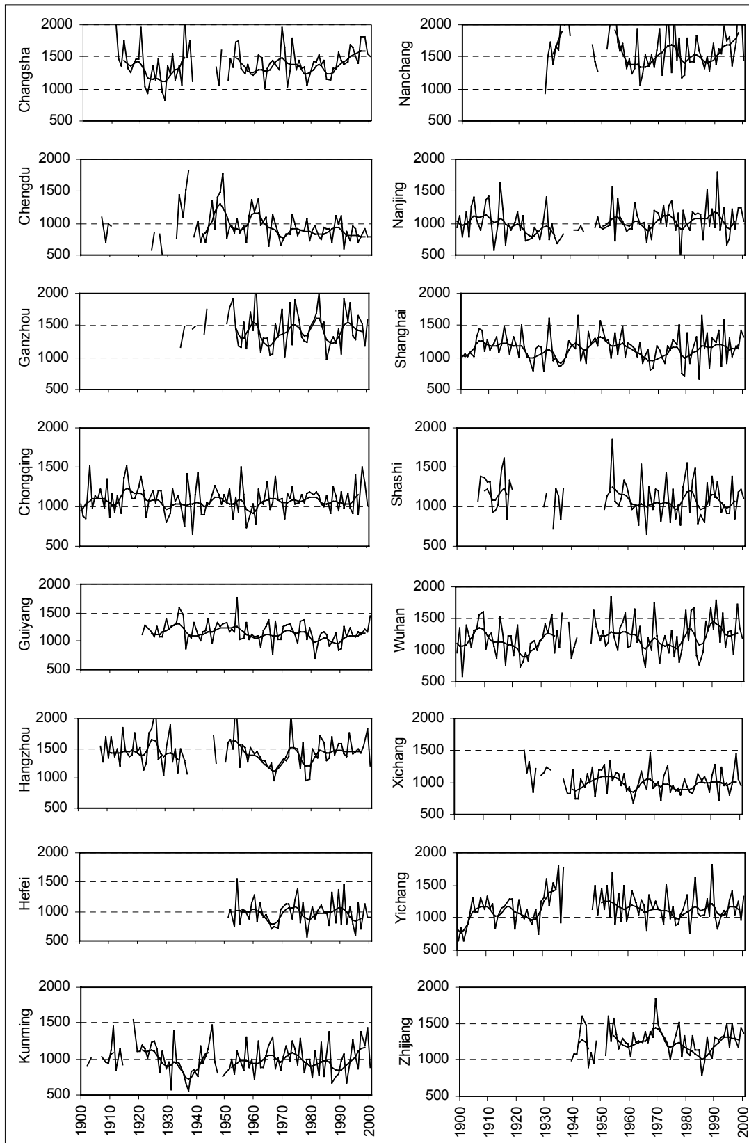
Figure 2: Annual precipitation (scale in mm) and filtered values Gauss low pass filter, based on 10 years time steps)
