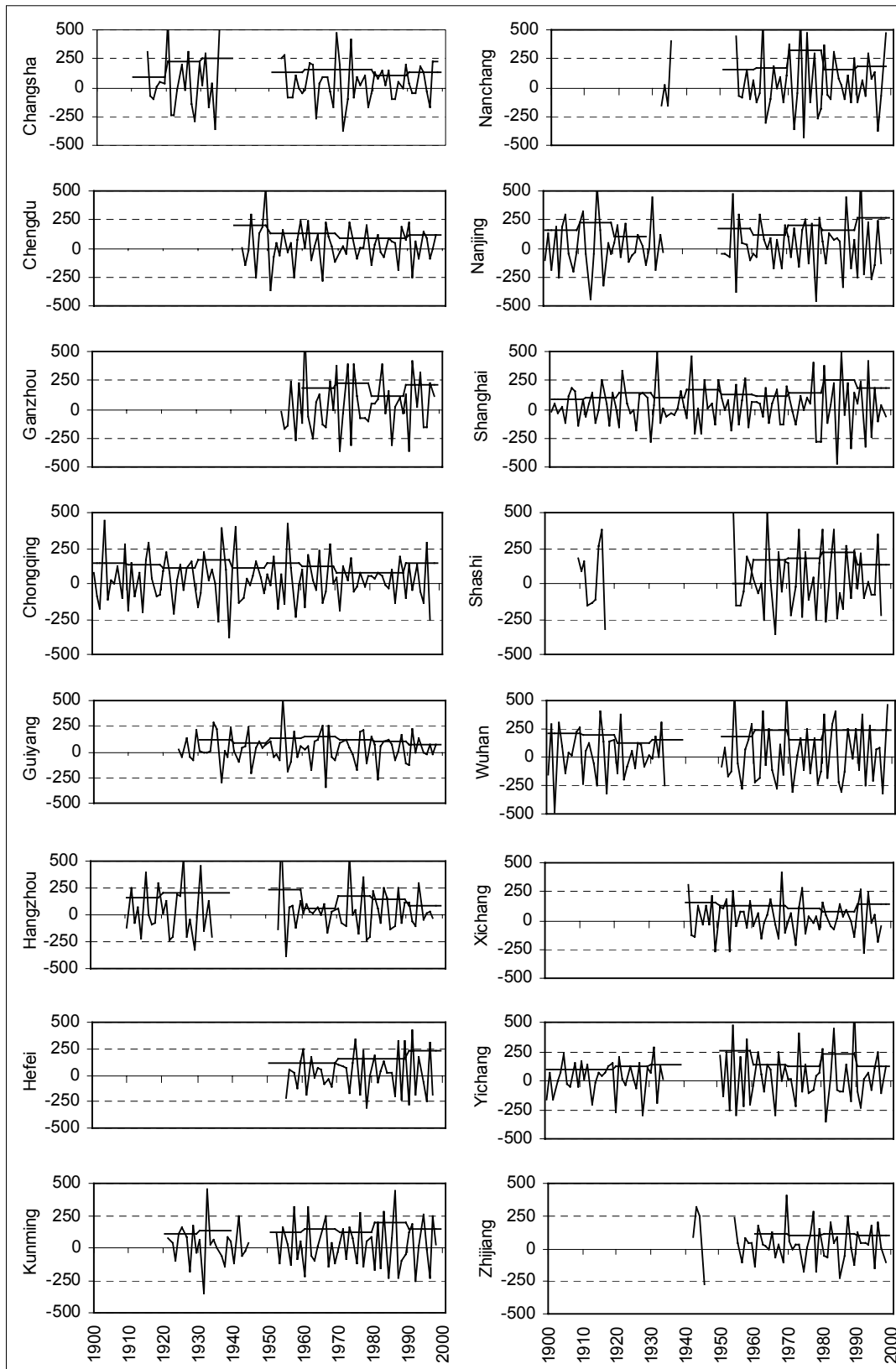
Figure 5: Gauss high pass filtered data of the annual precipitation (in mm, based on 10 years time steps), and their absolute decade averages (darker line)
