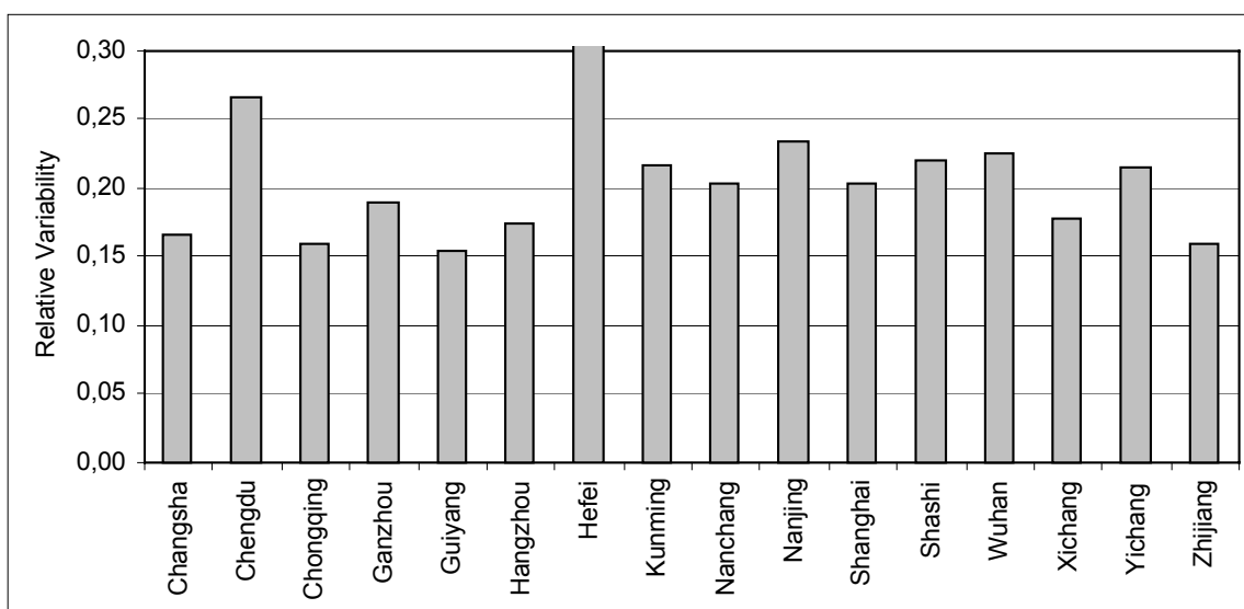
Figure 4: Relative variability of the annual precipitation sums from 1930 to 1999 in the Yangtze catchment
