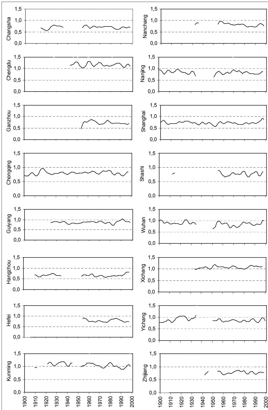
Figure 8: Inner-annual variability (s/x)
