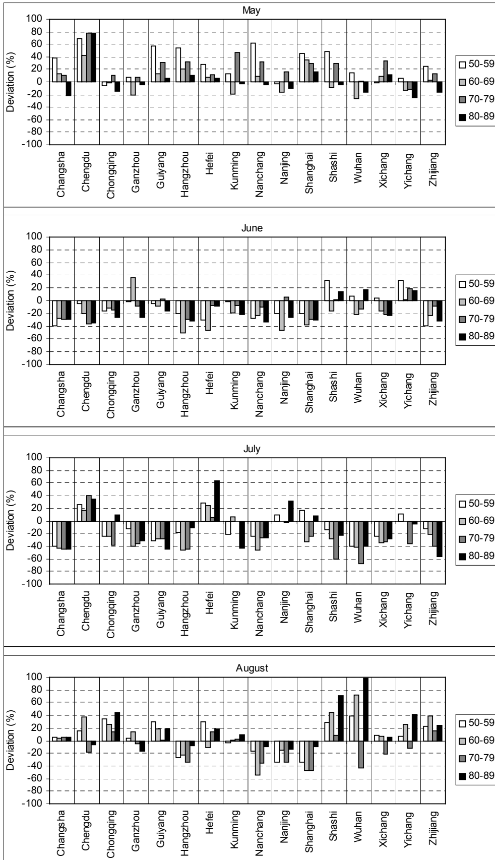
Figure 10: Deviation of the mean monthly precipitation of the 50s, 60s, 70s and 80s from the 90s average
