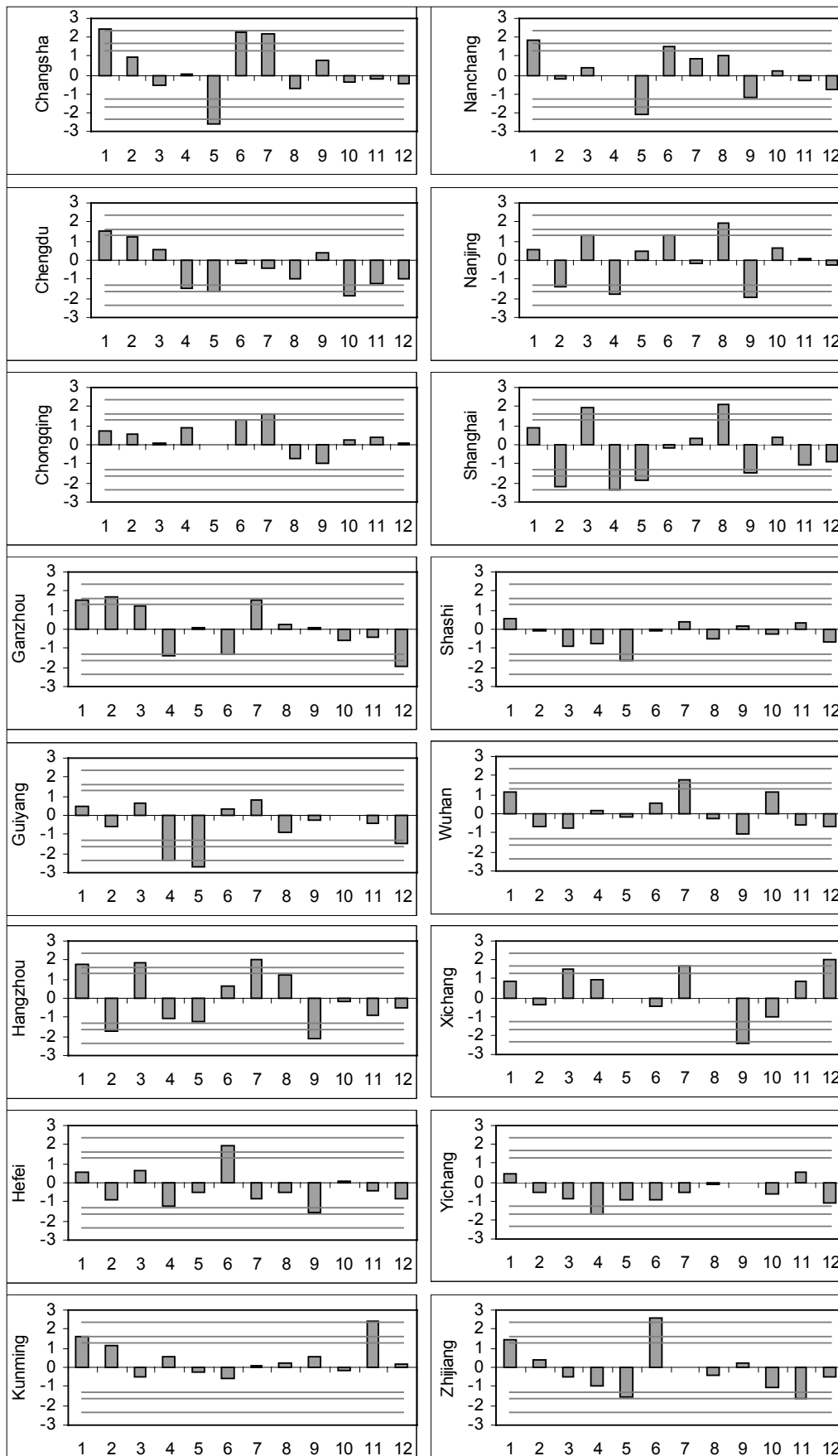
Figure 11: Mann-Kendall trend test for monthly precipitation 1950 – 1999
