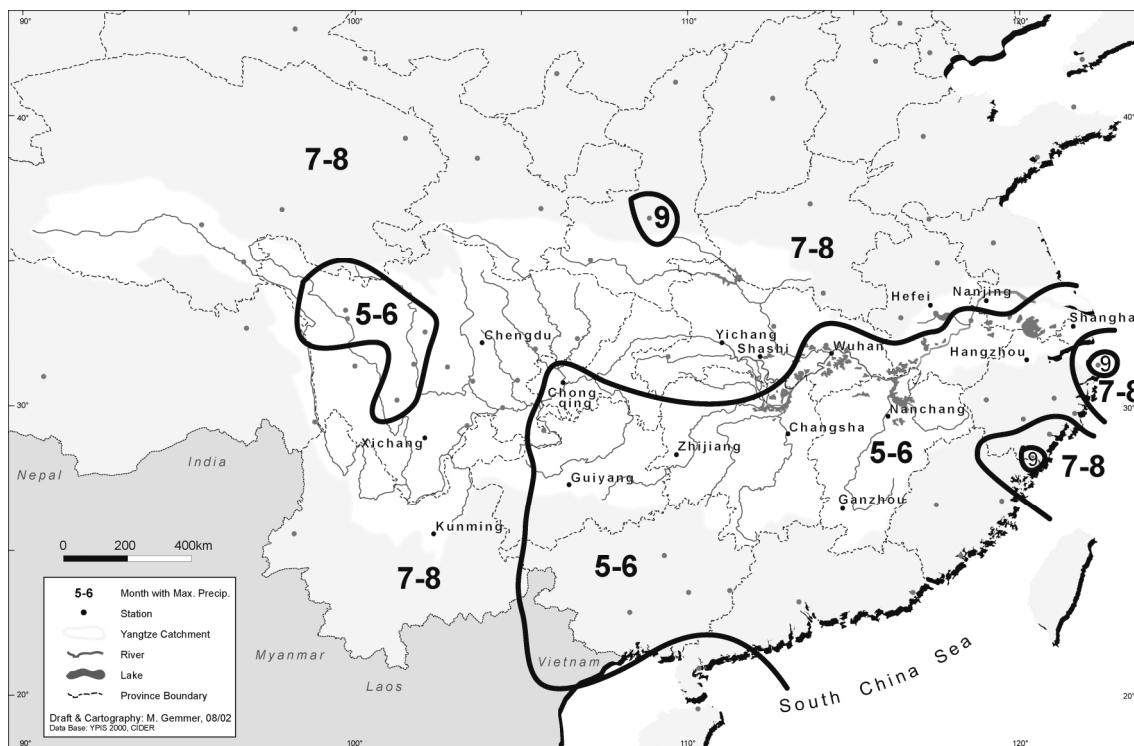
Figure 7: Months with maximum precipitation
