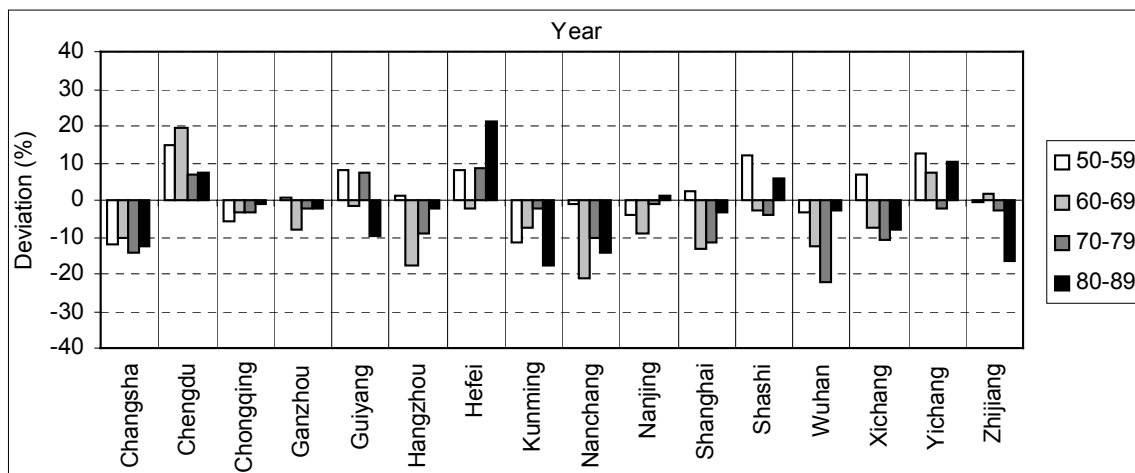
Figure 3: Deviation of the average annual precipitation of the 50s, 60s, 70s and 80s from the 90s average
