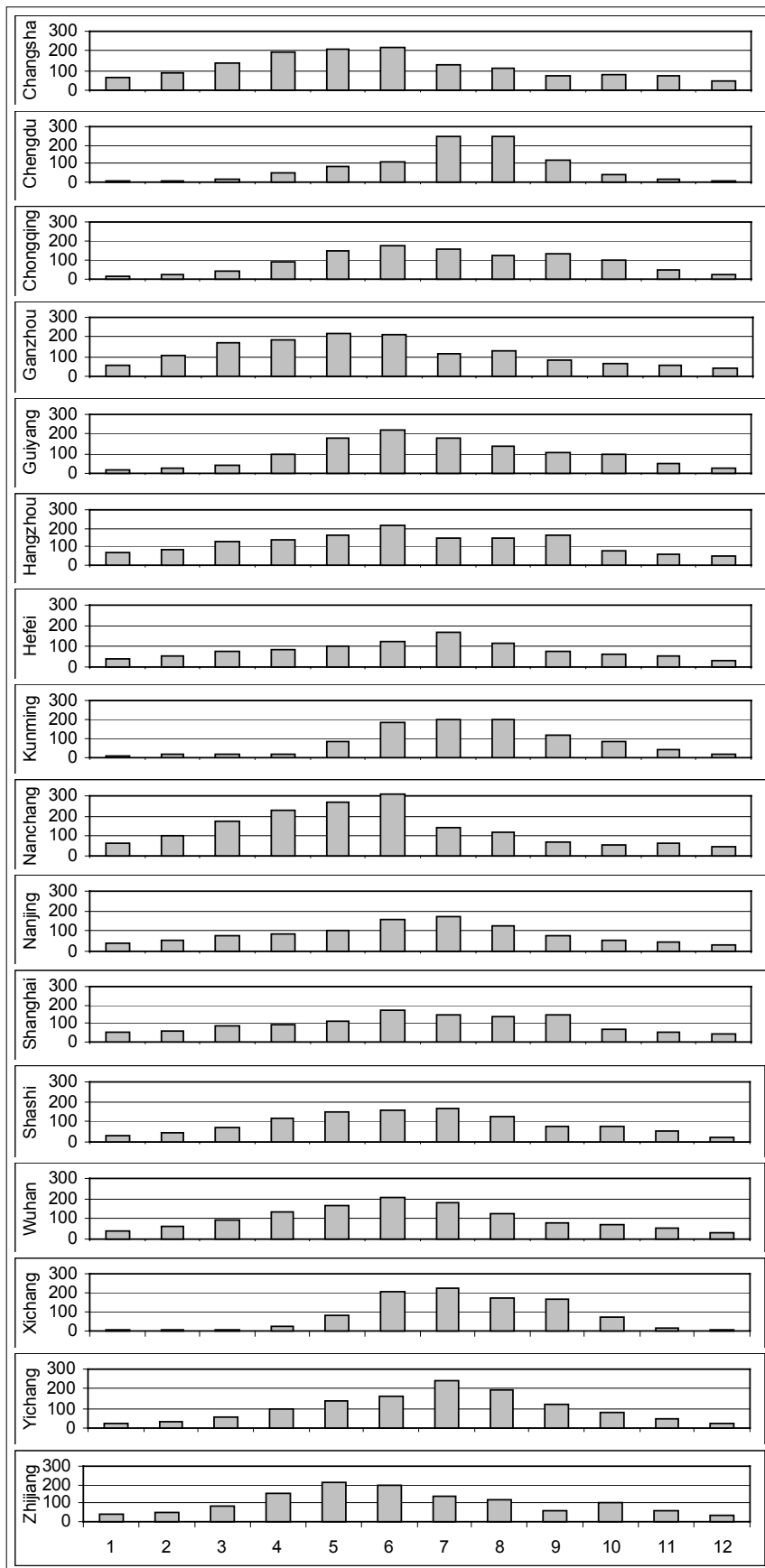
Figure 6: Monthly precipitation averages (mm, 1930 – 1999)
