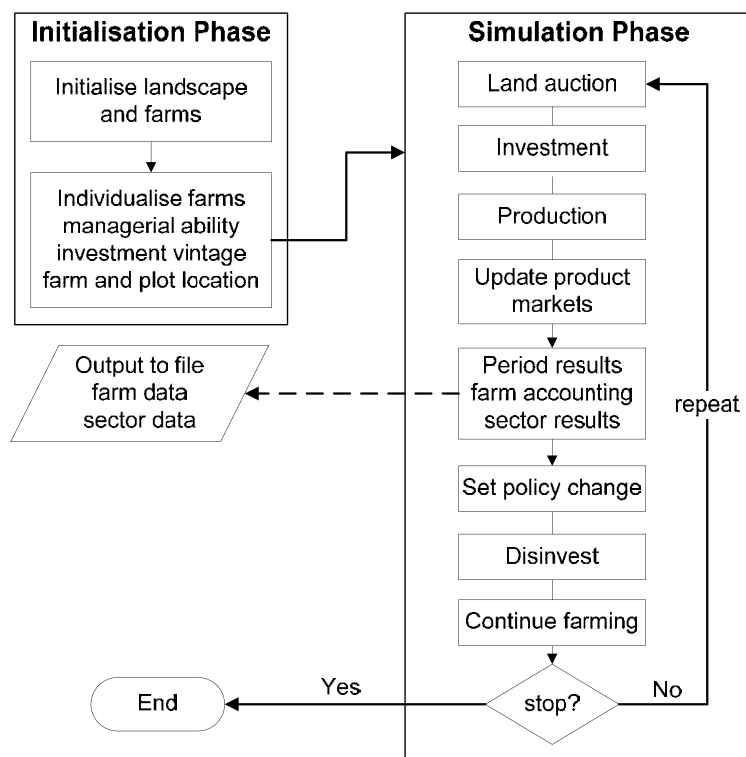
Figure 3-1: Sequence of operations in AgriPoliS
