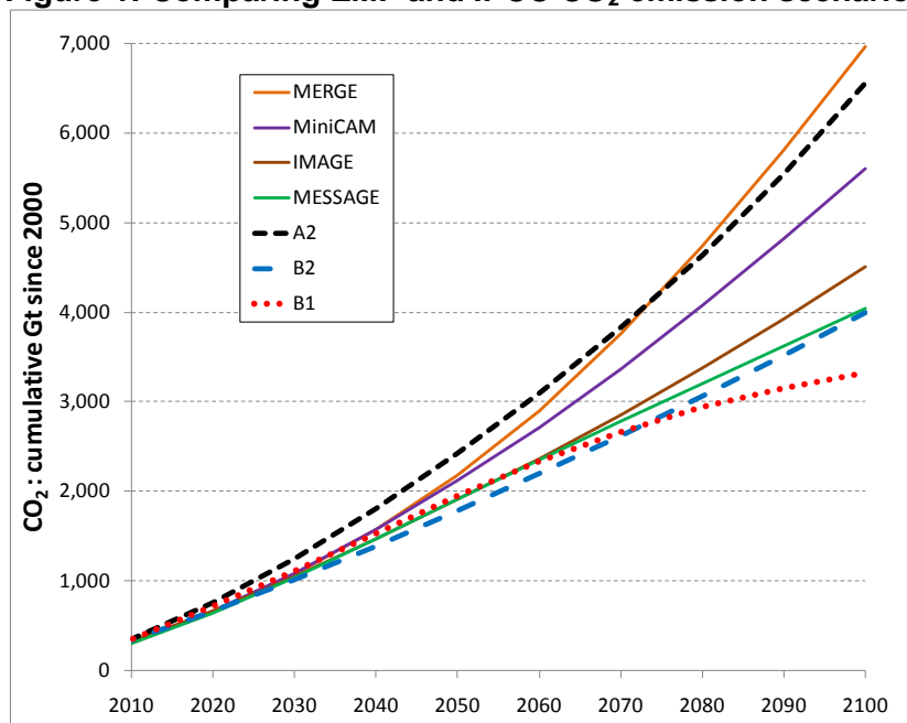
Figure 1: Comparing EMF and IPCC CO 2 emission scenarios
