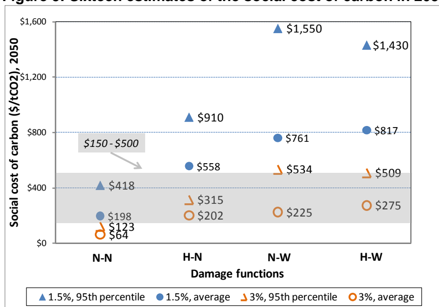
Figure 5: Sixteen estimates of the social cost of carbon in 2050
