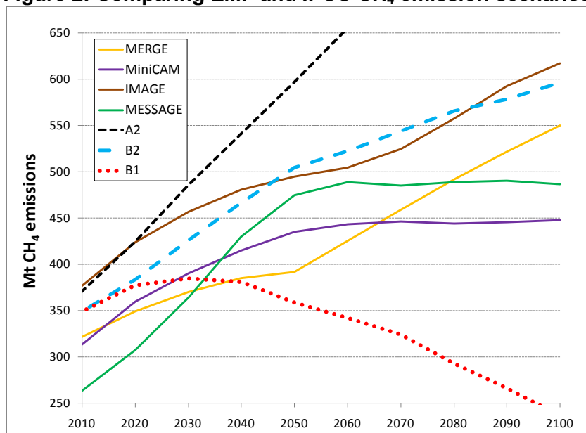
Figure 2: Comparing EMF and IPCC CH 4 emission scenarios
