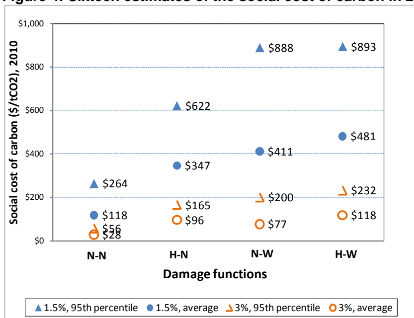
Figure 4: Sixteen estimates of the social cost of carbon in 2010
