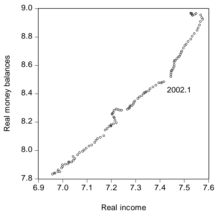
Figure 2 Structural break in income elasticity
