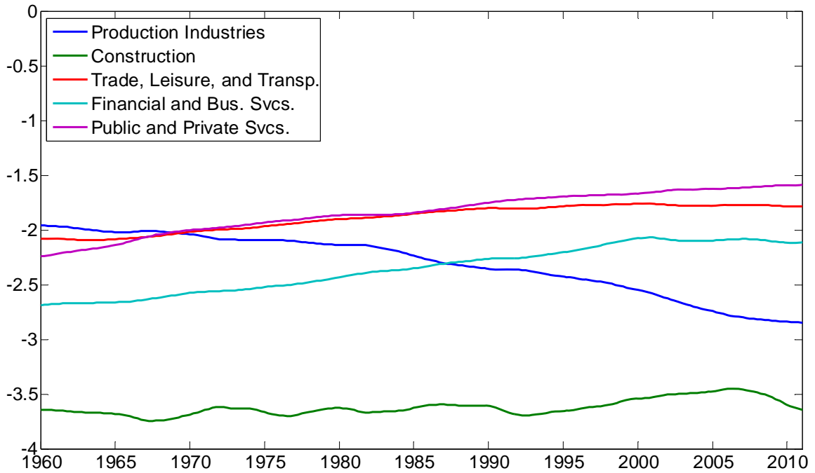
Figure 3: Posterior mean employment trends (United States, 5 sectors)
