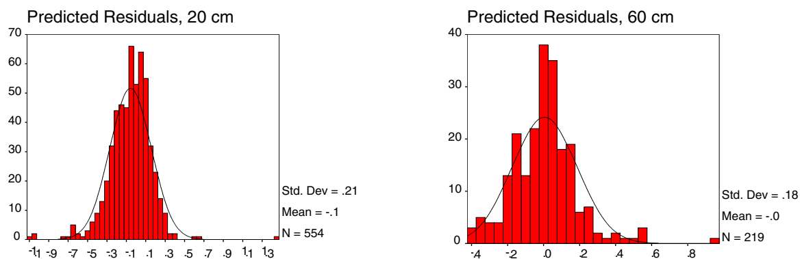
Figure 2: Histograms of the predicted residuals for the upper (left) and the lower layer (right)
