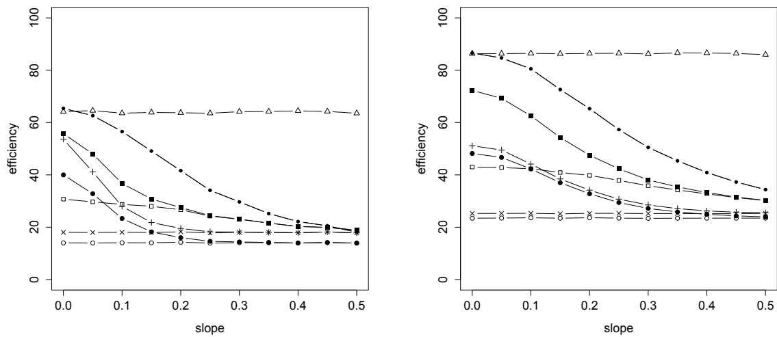
Figure 3: Relative efficiencies for Gaussian noise, autocorrelations \rho = 0.0 (left) and \rho = 0.6 (right): median ( \cdot ), RM ( \triangle ), PFMH ( \times ), CFMH ( + ), PRMH ( \circ ), CRMH ( \bullet ), PRMMH ( \square ) and CRMMH ( \blacksquare ).
