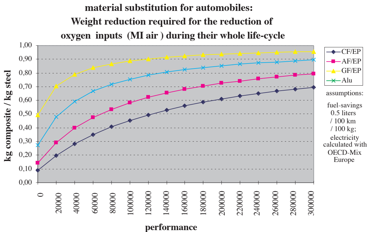
Fig.10.2: Material substitution for automobiles: Weight reduction required for the reduction of air (oxygen) inputs during their whole life-cycle; without inputs for material manufacturing Source: own calculations
