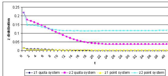
Figure 5: Ability distribution, z_1 and z_2 .
