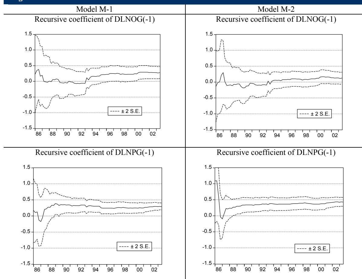
Figure 5. – Estimated recursive coefficients
