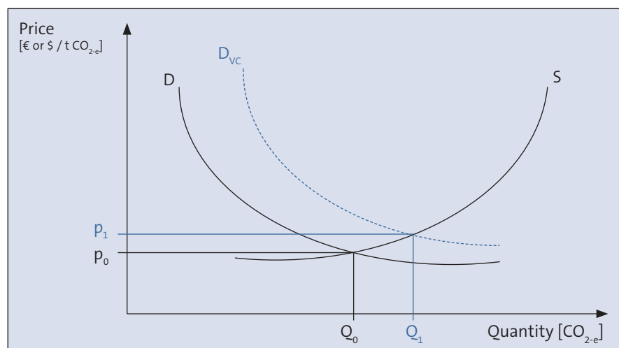
Figure 9: Qualitative effects of voluntary compensation on market prices under the Kyoto System/EU ETS
