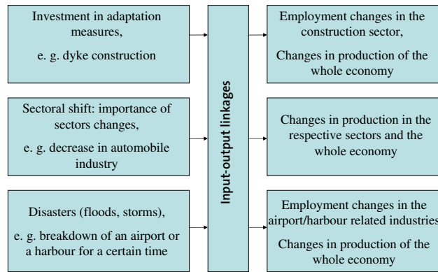
Figure 2: Input-Output linkages
