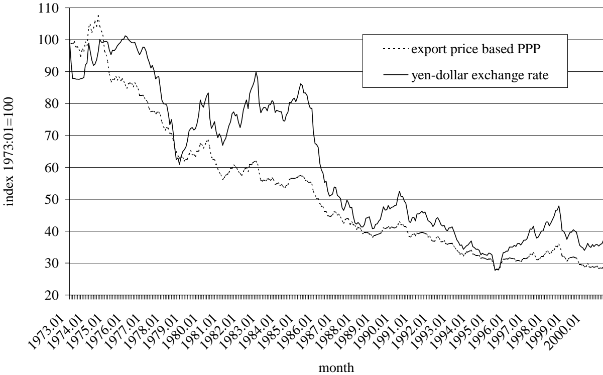
Figure 3: Yen-Dollar Exchange Rate and Export Price Based PPP
