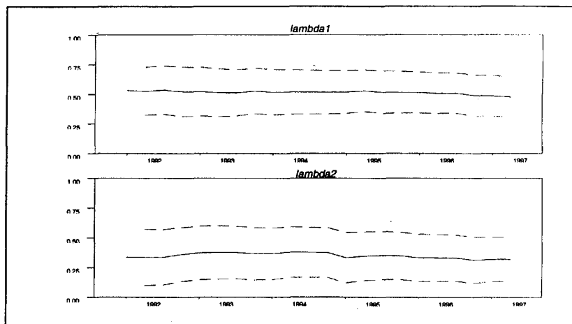
Figure 2 - The eigenvalues
