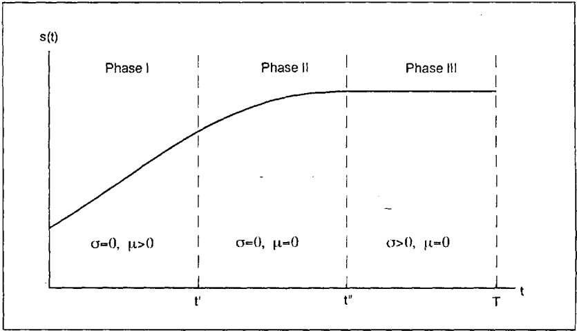
Figure 1. Optimal Accumulation of Greenhouse Gases.
