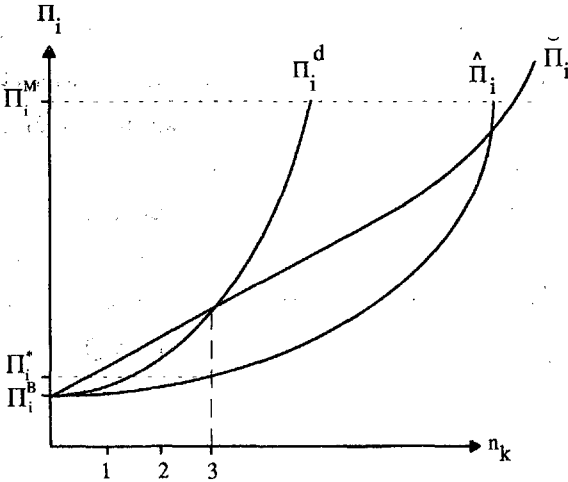
Figure 2: \Pi_i^B < \Pi_i^* < \Pi_i^M
