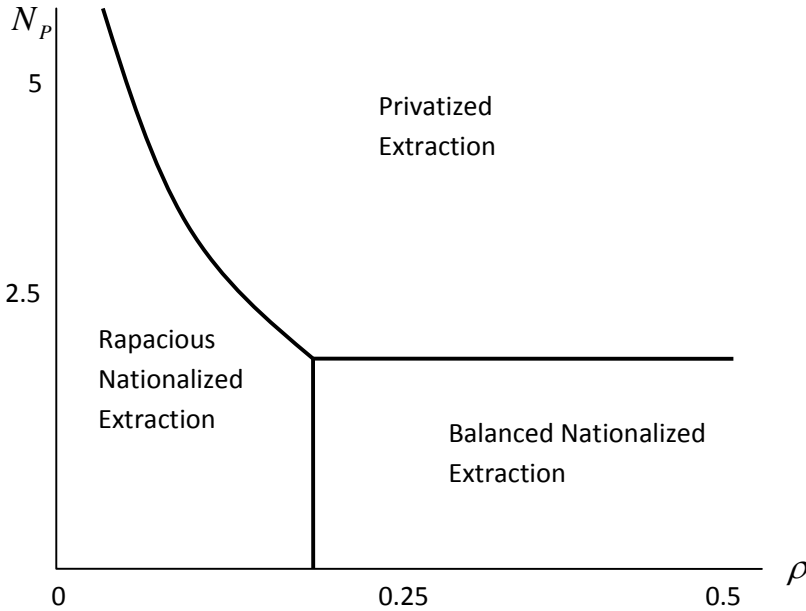
Figure 4: Extraction regimes
