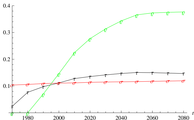
Figure 9: Predicted policies for Japan: \tau_t (black), \sigma_t (red), \rho_t (green).
