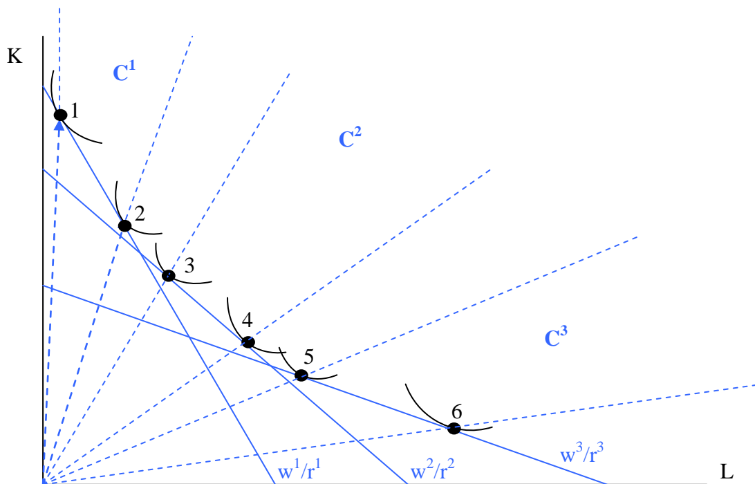
Figure 4: Multi-cone specification
