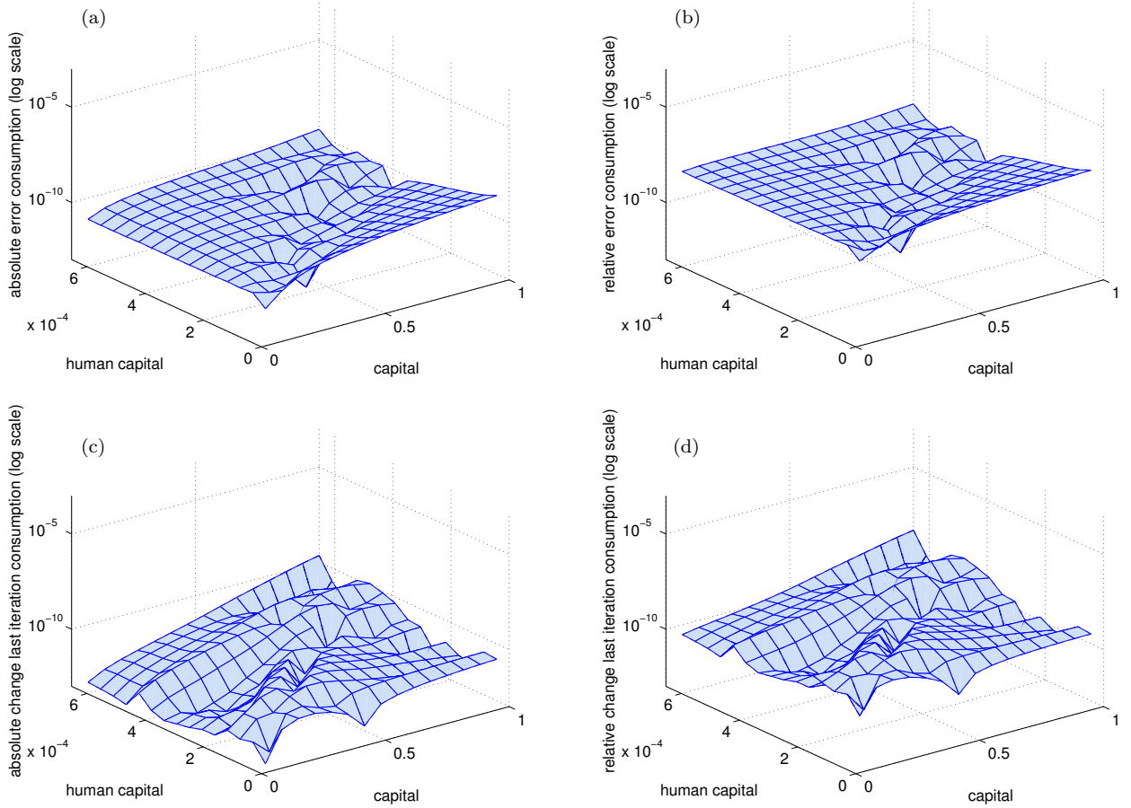
Figure 8: Absolute and relative error compared to the analytical benchmark solution and to the policy function of the last iteration
