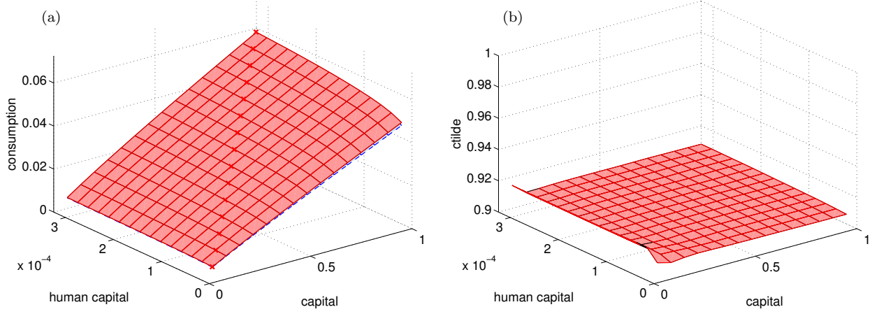
Figure 11: Policy functions and optimal jump for consumption in the Lucas model (2)
