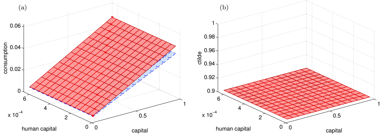
Figure 7: Policy functions and optimal jump for consumption in the Lucas model (1)
