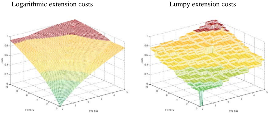
Figure 5: Global cost function, six-node network, fixed reactances
