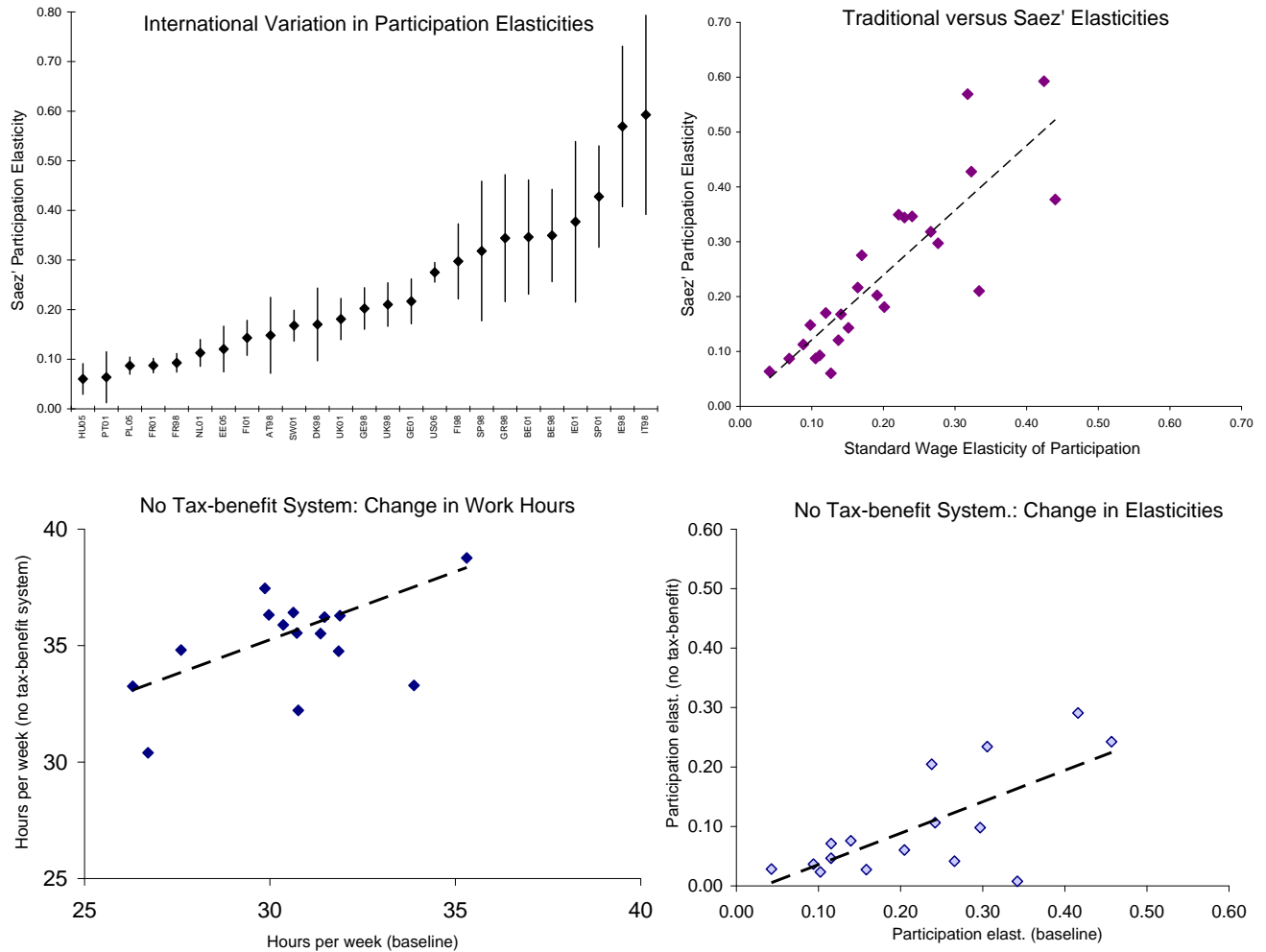
The top-left panel represents Saez' participation elasticities averaged over income groups i=1,\dots,l (point estimates) and 95% bootstrapped confidence intervals. The top-right panel compares these elasticities with traditionally defined participation elasticities. Lower panels describes a situation with no tax-benefit system (change in hours and participation elasticities).
