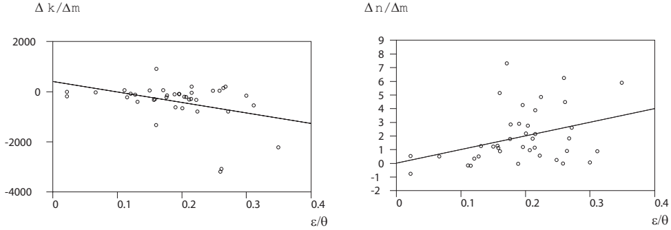
Figure 1: The response of per capita capital k and population growth n to change in mortality as a function of \varepsilon/\theta .
