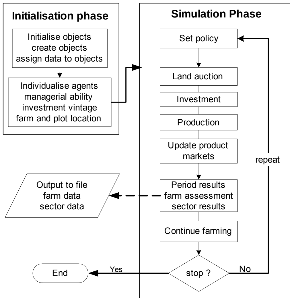
Figure 3-5: Model dynamics implemented in the Manager class
