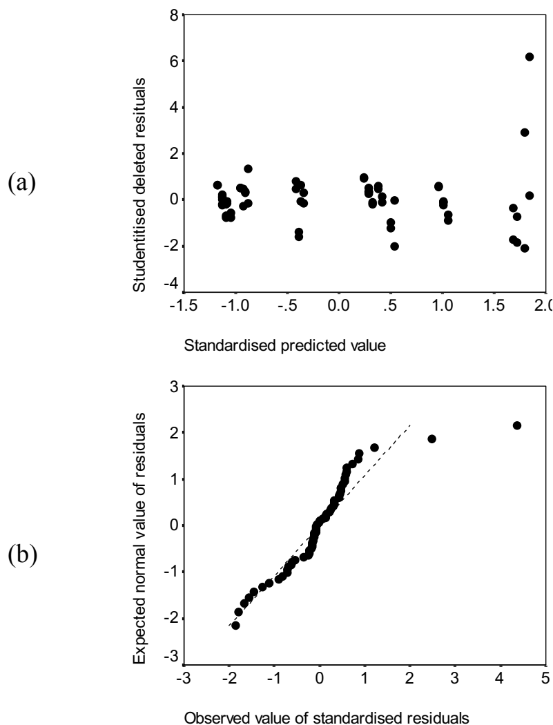
Figure 5-5: Residual plots. (a) Scatter plot of studentitised deleted residuals versus standardised predicted values; (b) Q-Q normal probability plot
