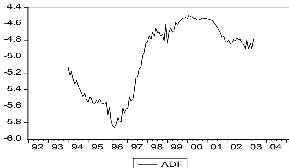
Figure 3: Recursively estimated Gregory – Hansen ADF statistics
