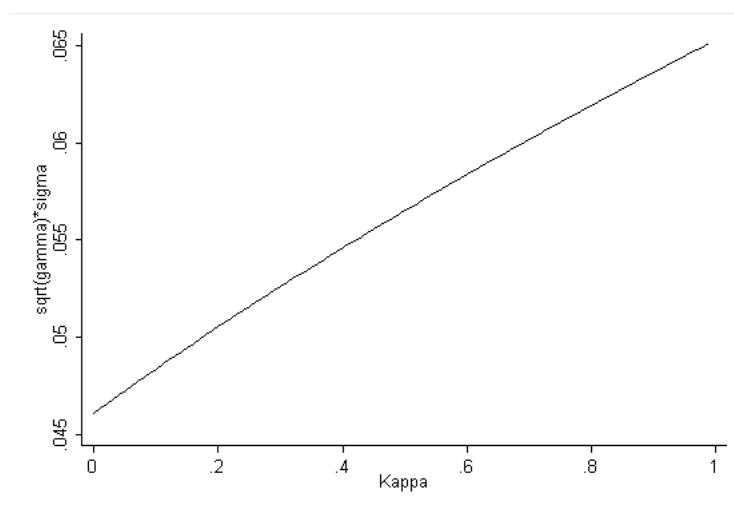
Figure 1: Two parameter sensitivity analysis for the DID estimates in Meyer et al. (1995). Autocorrelation in group-time shocks and allowed standard deviation of the group-time shocks.
