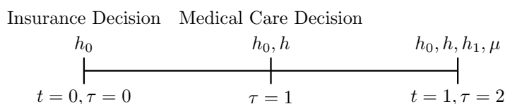
FIGURE 1. Decisions schedule and information
