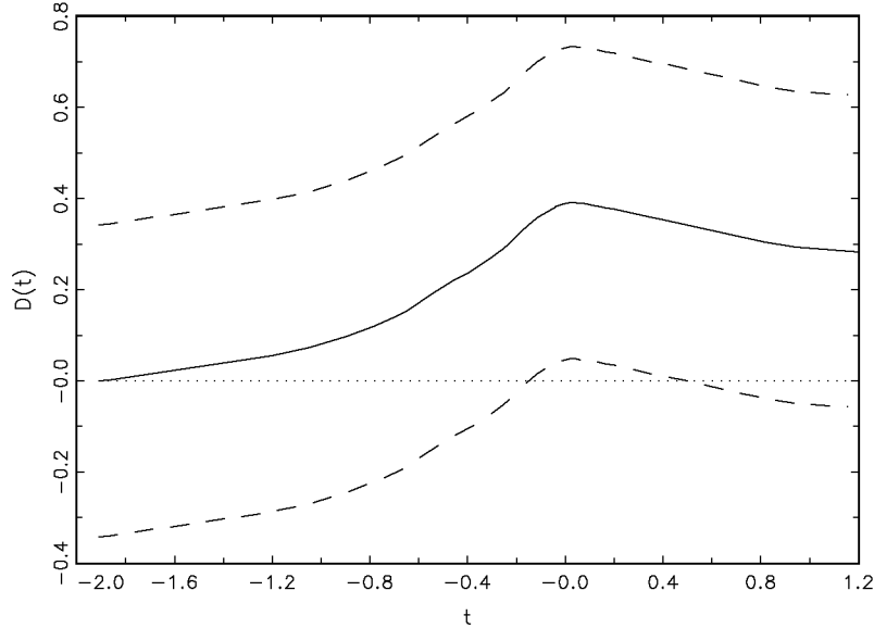
Figure 1: \hat{\mathcal{D}}_{n,m}(t) with bootstrapped 95 %-confidence band ( F(x) = \Phi(x) , G(x) = \Phi(5x) , n = m = 25 , B = 500 )
