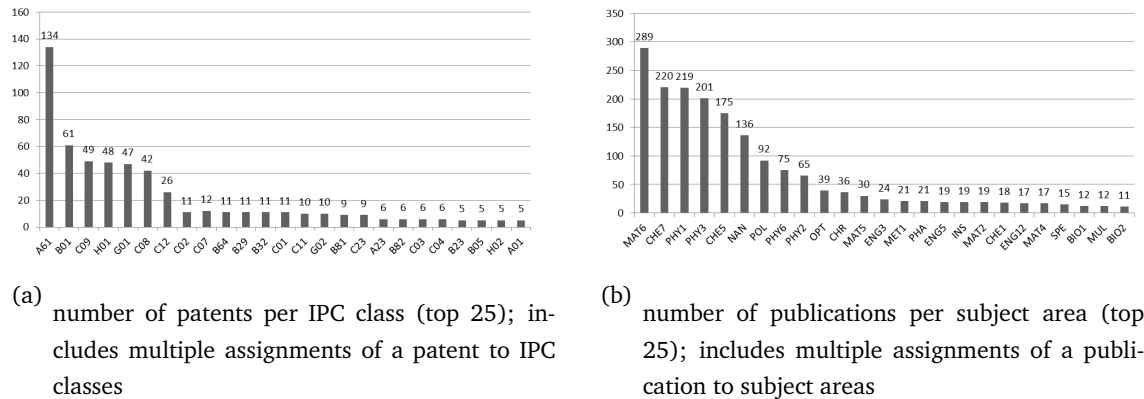
Figure 2: Specialization and diversification of the NKB in Hamburg (see tables 5 and 4 for decoding of the labels for the IPC classes and the subject areas)
