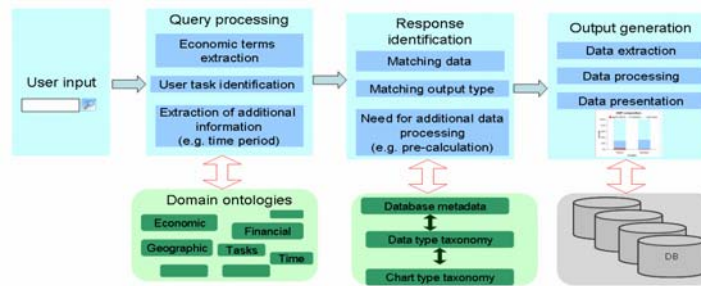
Figure 3: System framework
