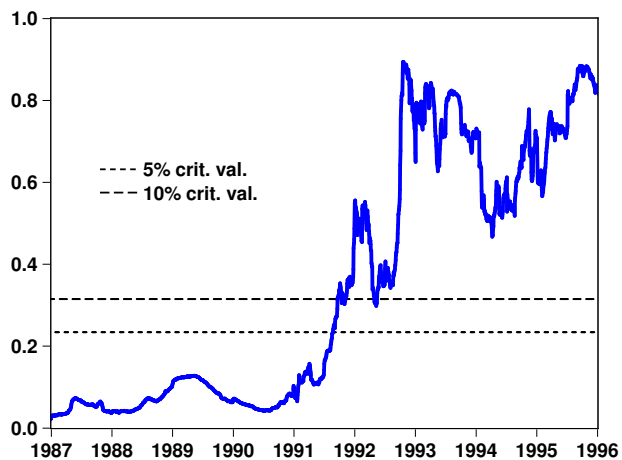
Figure 2: Detection of break point using test for change in persistence
