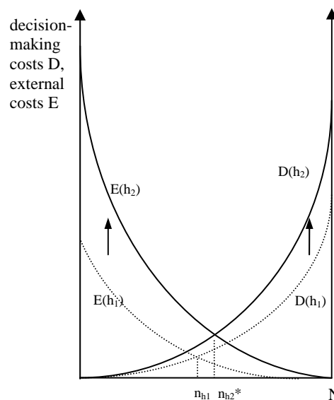
Fig. 4 A more inclusive decision-rule is optimal.
