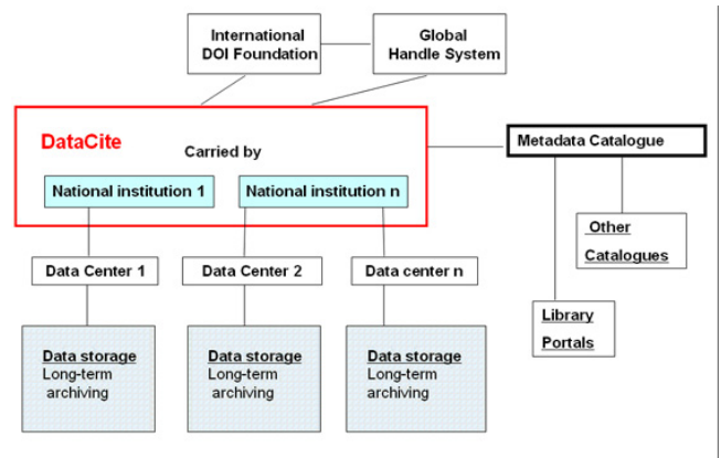
Figure 3. The overall structure of DataCite
