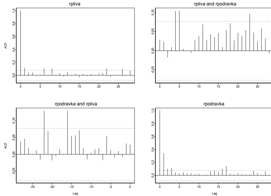
Figure 2: Correlograms and cross-correlograms between Pliva and Podravka square returns
