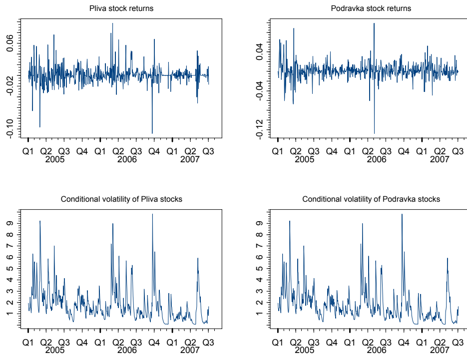
Figure 3: Returns of Pliva and Podravka stocks with their conditional volatilities
