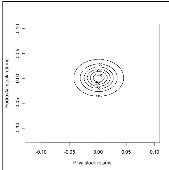
Figure 1: Contour plot of the Bivariate Student's t-distribution Density ( df = 3.2 )
