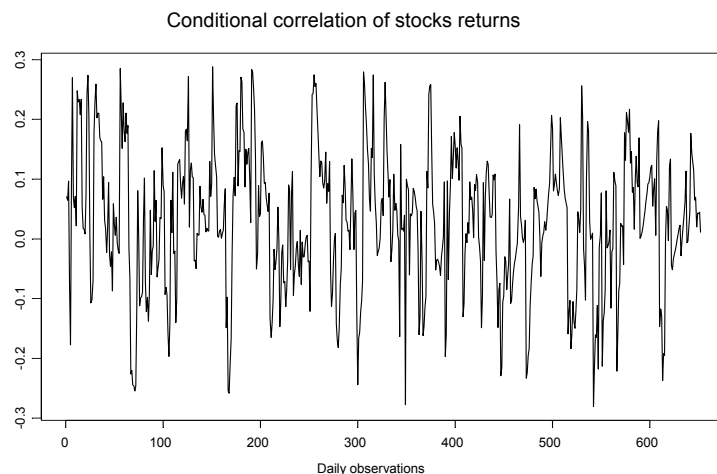
Figure 4: Conditional correlation of Pliva and Podravka stock returns
