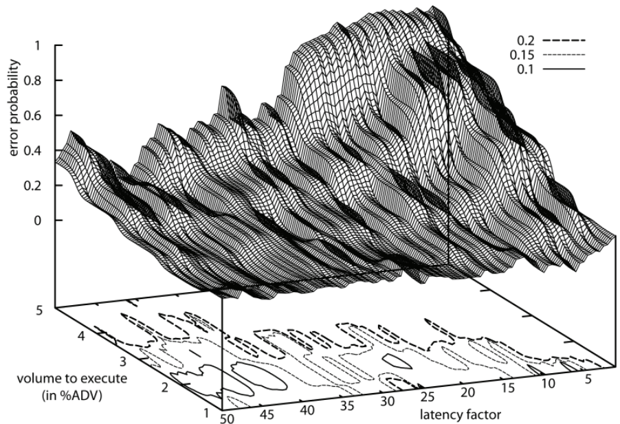
Figure 3. Error probability for rejecting H_0 when using an algorithmic trader agent following strategy B (interpolated)
