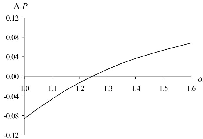
Figure 3: Change of the P index, upon revision of the income distribution from I_0^t = \{2, 3, 6, 7\} to I_1^{t+1} = \{5, 5, 8, 8\} , as a function of \alpha \in [1, 1.6]
