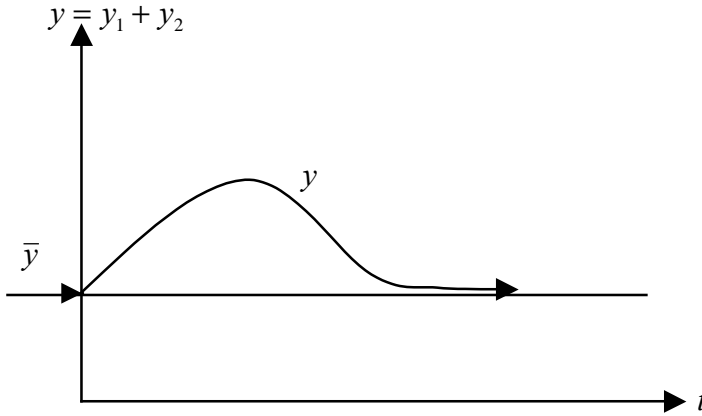
Figure 11: Response of aggregate output to dm > 0 with lagged output adjustment
