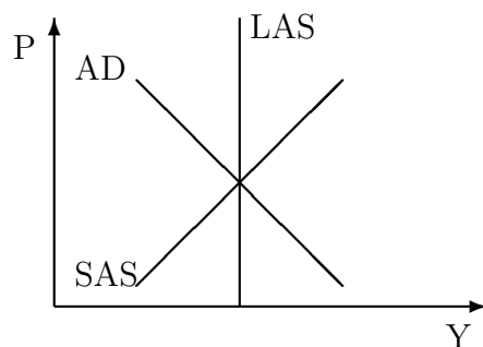
Figure 2: AS-AD diagram
