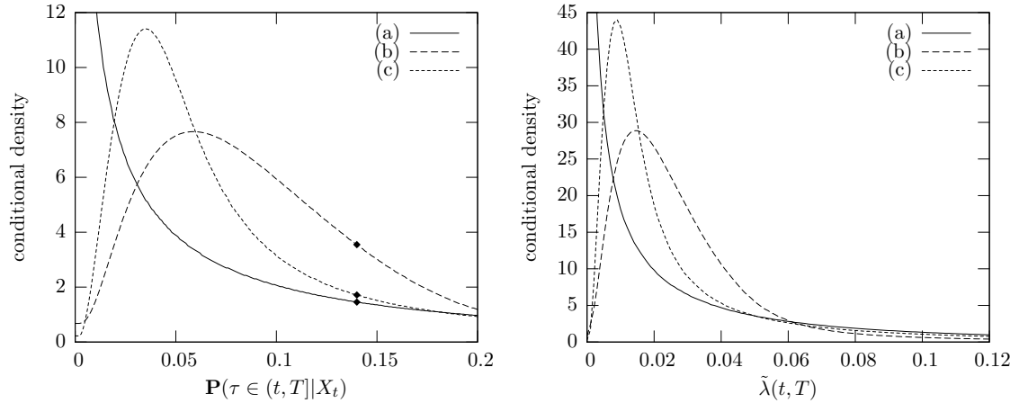
Figure 4: Distributions of P(t, T) (left) and \tilde{\lambda}(t, T) (right) conditional on \{\tau > t\} for different dynamics. We choose t = 1, T = 5 and an initial hazard rate of 3%. The diamonds mark the initial 5-year default probability. The parameters are given in Table 1.
