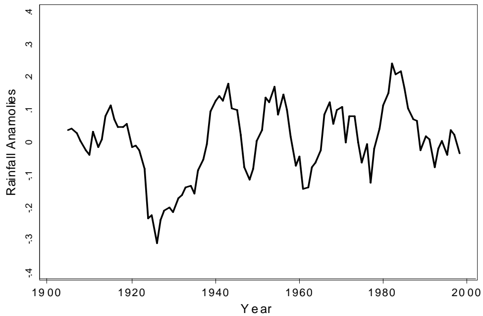
Figure 2: Rainfall in Non Sub-Saharan African Countries – Long Term Trends
