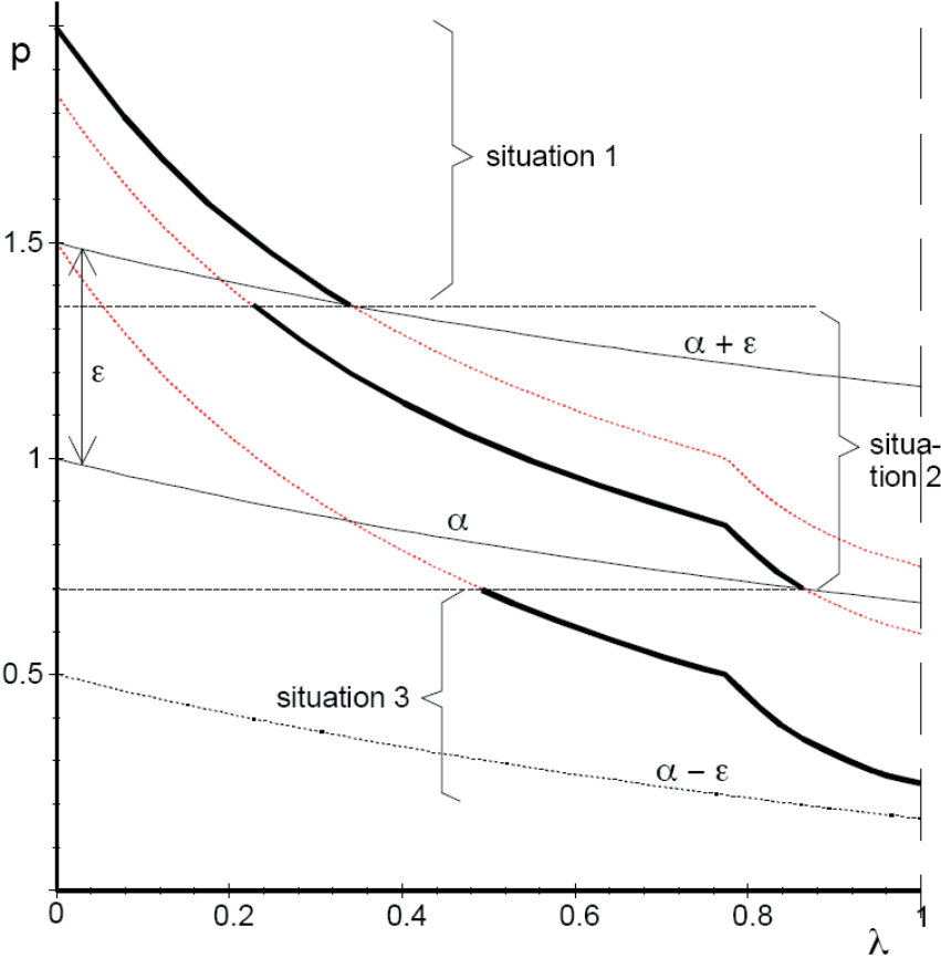
Fig. 2: Illustration of “long-term” Nash bargaining \lambda \frac{W}{K} under uncertainty ( \eta = 1/2, \theta = 1/4, W = 1/2, \varepsilon = 1/2, \delta = 9/10 )
