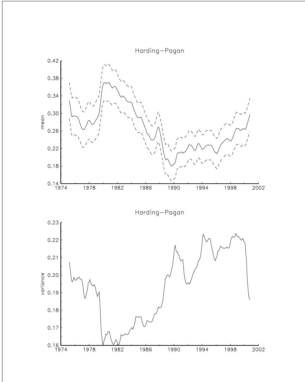
Figure 4: GMM estimates of m_t and v_t^2 , the former alongside their 95% confidence intervals. Estimates are computed using a rolling window of 14 years.
