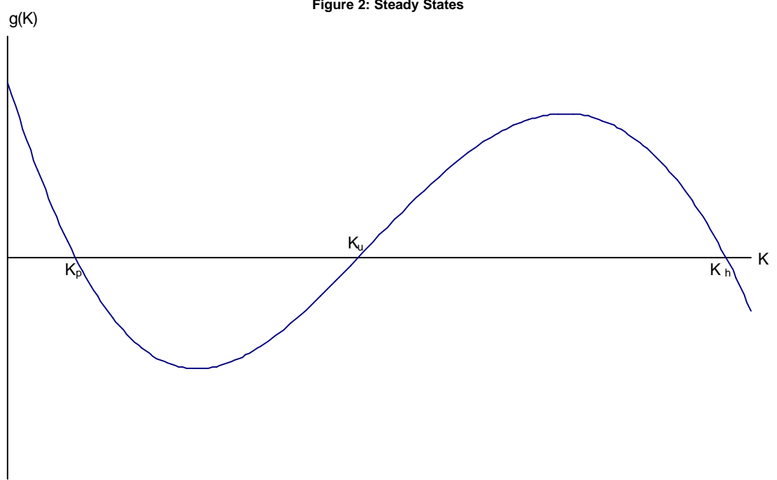
Figure 2: Steady States
