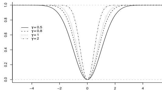
Figure 4: ESTAR: Transition function for different \gamma .
