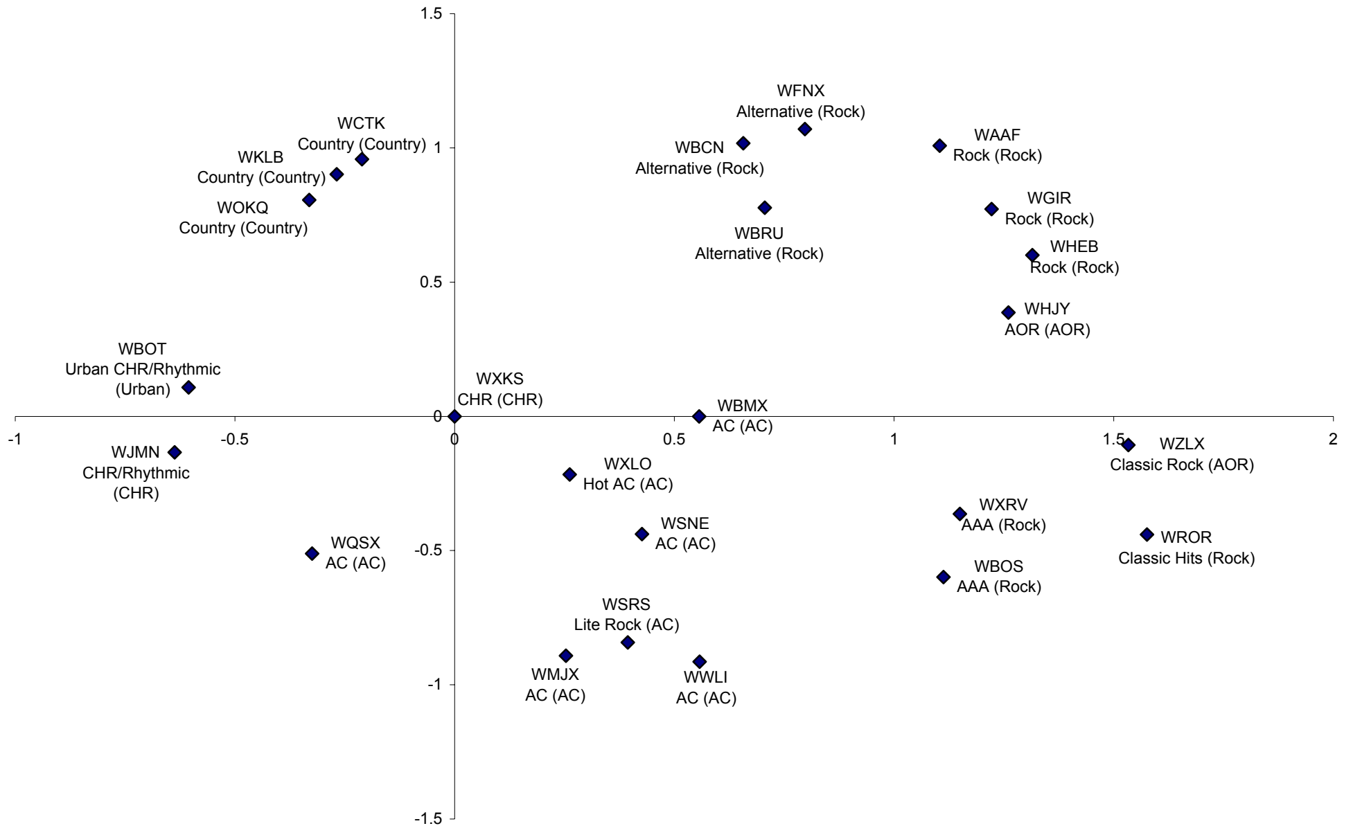
Figure 3: Location of Stations Rated in Boston based on their First Week of November 2001 Playlists and Measure 1 (Each Artist Defines a Separate Dimension of Product Space) Pair Distances with Station Formats and (Categories)
