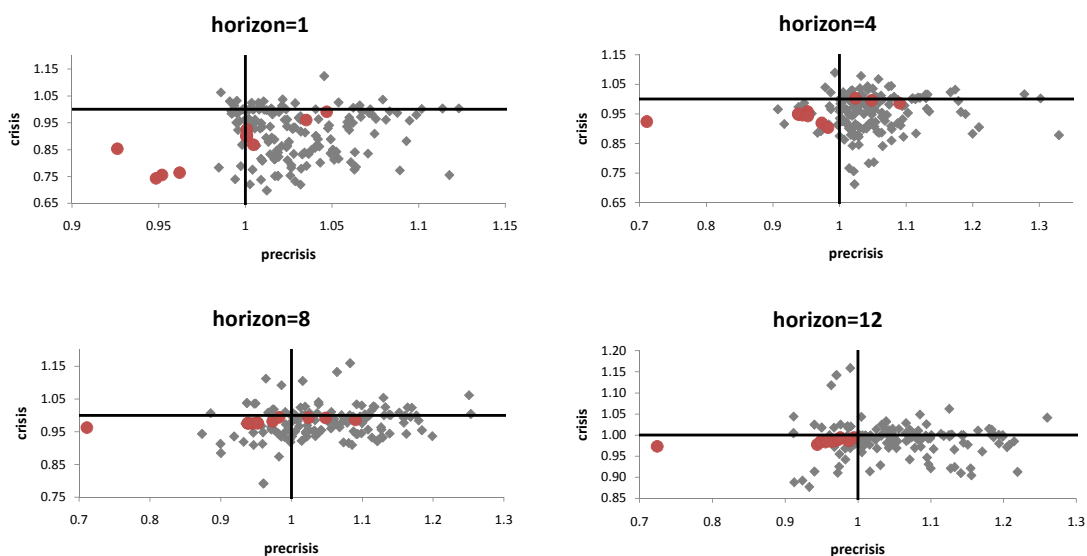
Figure 3: Out-of-sample stability for IP
