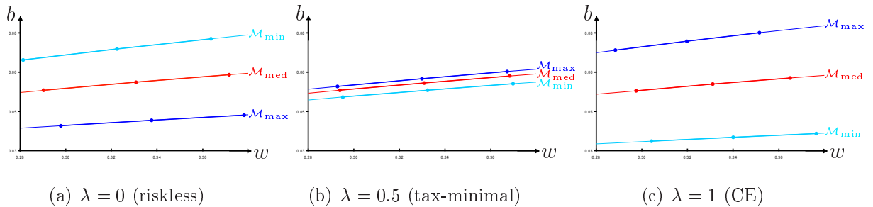
Figure 3: Stable sets \mathcal{M}_{\min} := \mathcal{M}_{\varepsilon_{\min}}^{\theta_\lambda} , \mathcal{M}_{\text{med}} := \mathcal{M}_{\varepsilon_{\text{med}}}^{\theta_\lambda} , \mathcal{M}_{\max} := \mathcal{M}_{\varepsilon_{\max}}^{\theta_\lambda} .
