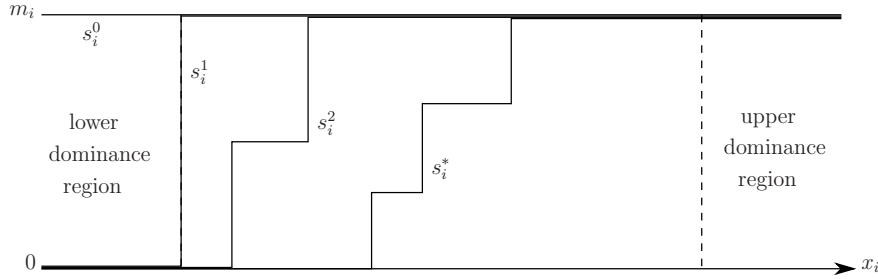
FIGURE 1. The strategy of player i in an upper-best reply iteration leading to the greatest equilibrium strategy profile s^* .
