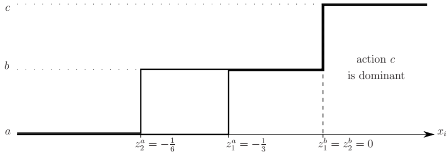
FIGURE 11. (a, a) is attained from above under f in \bar{e}(g, f) .
