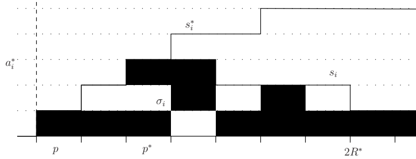
FIGURE 14. Robustness implies existence of a mixed strategy profile \sigma that prescribes a^* with positive probability. An upper-best reply iteration from the mixed strategy profile \sigma yields the pure strategy profile s . The greatest equilibrium s^* \geq s is constant for signals greater than 2R^* .
