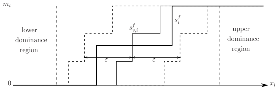
FIGURE 2. s_i^f and s_{v,i}^f for v < \bar{v}
