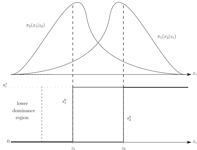
FIGURE 4. TOP: The thresholds z_i , at which players believe that the opponent will receive a signal x_{-i} \geq z_{-i} with probability \frac{1}{2} . BOTTOM: The starting point for the upper-best reply iteration.
