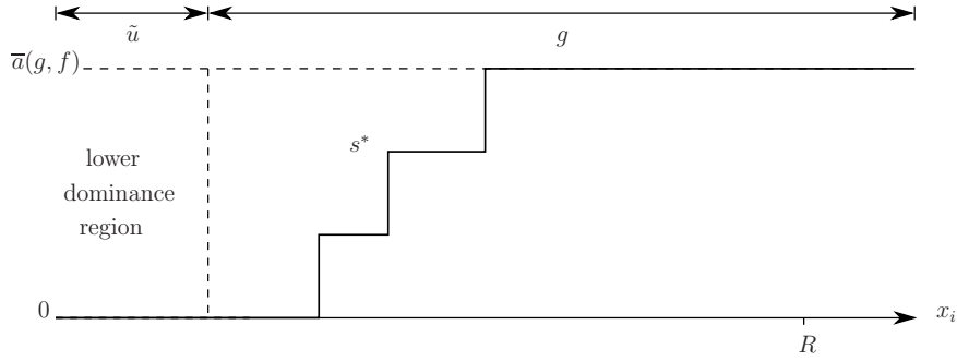
FIGURE 3. A lower- f -elaboration such that the greatest equilibrium strategy profile, s^* , attains \bar{a}(g, f) .
