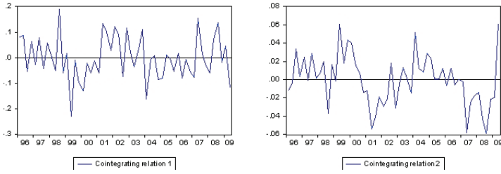
Figure 1: Cointegration relations (1995:1-2009:2)
