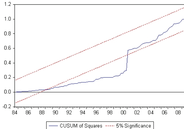
Figure 6: CUSUM of Squares of the ARDL model (1980:1-2009:2)
