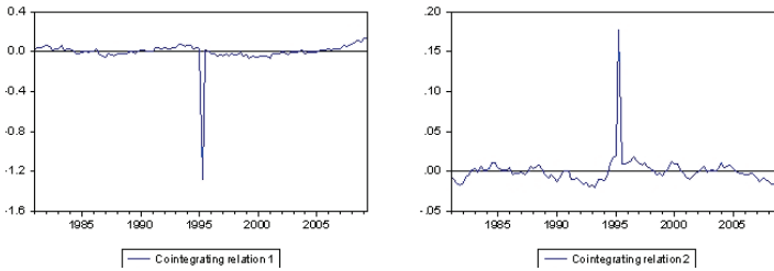
Figure 2: Cointegration relations (1980:1-2009:2)
