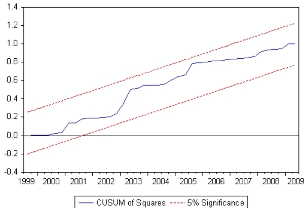
Figure 5: CUSUM of Squares of the ARDL model (1995:1-2009:2)
